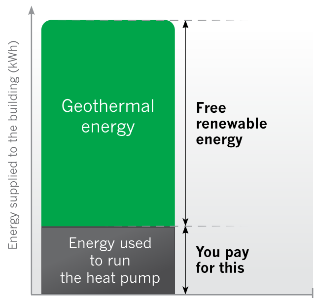
This graphic shows the building's total energy consumption for heating and hot water. The grey area shows the energy used to run the heat pump. The calculation was made for a building of 1 000 m 2 in an average weather year.
